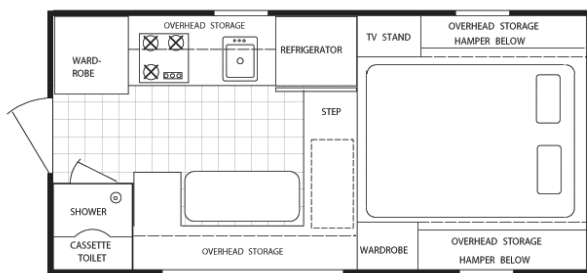
Laredo SC w/ Extended Cabover
